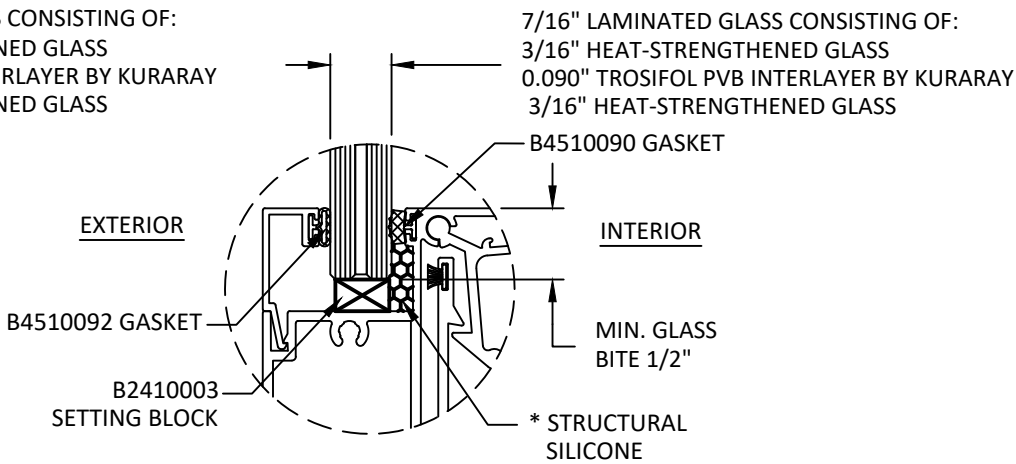
GLAZING DETAIL 2
