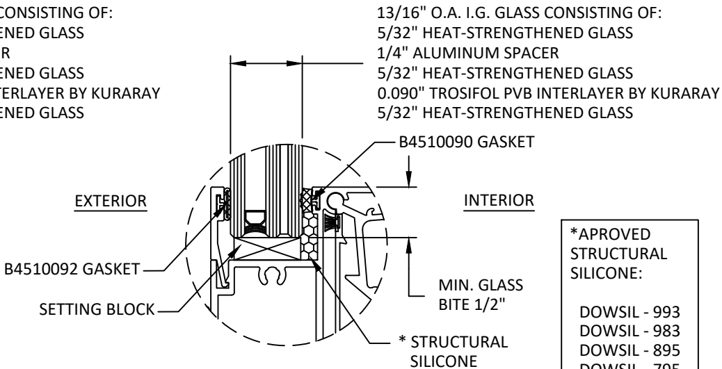
GLAZING DETAIL 4
